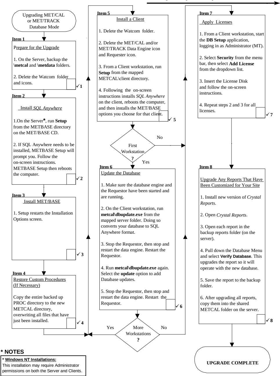
FLOWCHART 4 UPGRADING A NETWORKED DATABASE MODE MET/CAL 4.2, MET/TRACK 4.x OR MET/BASE 5.x
